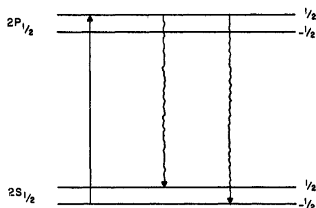
Figure 1. Absorption with \Delta M = +1 and spontaneous emission.
